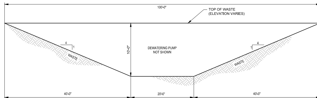
5 6 DEWATERING SUMP DETAIL NOT TO SCALE
