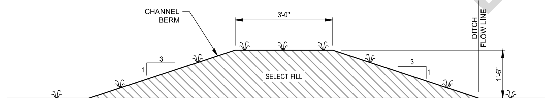
4 6 CHANNEL BERM NOT TO SCALE
