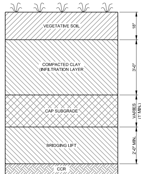
1 6 CLAY CAP DETAIL NOT TO SCALE
