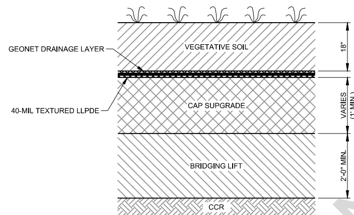
2 6 GEOCOMPOSITE CAP DETAIL NOT TO SCALE
