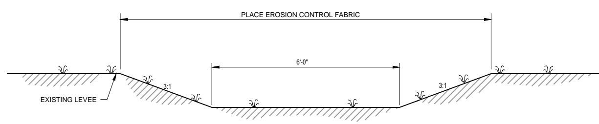
C 7 SECTION NOT TO SCALE
