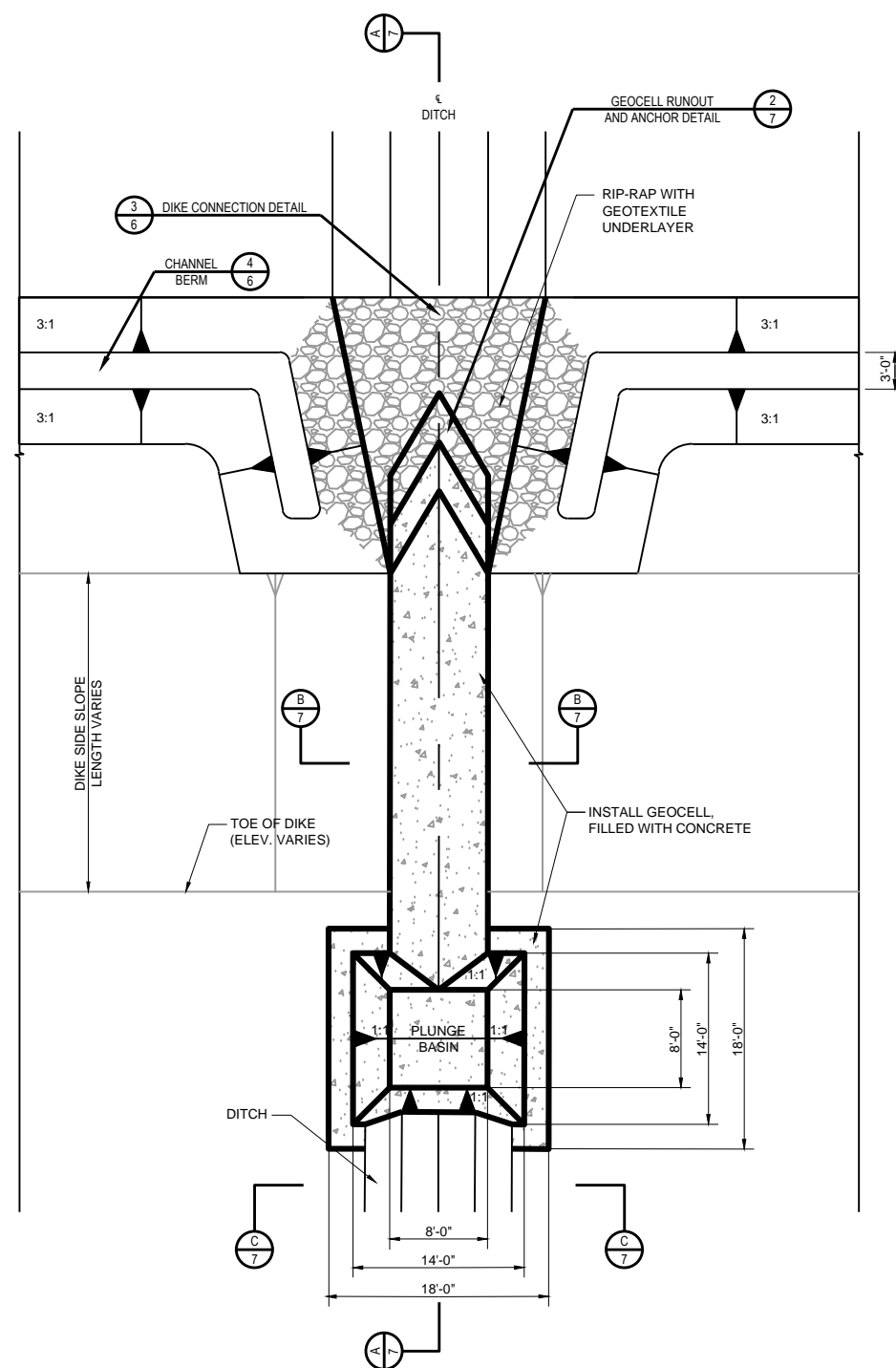
1 7 STORMWATER LET-DOWN STRUCTURE SCALE: 1"=20'
